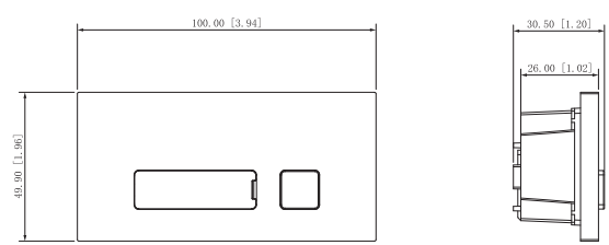
DHI-VTO4202F-MB1
